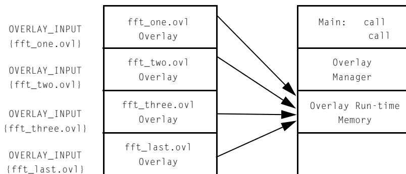
Figure 5-8. Example of Overlays – Not Grouped
