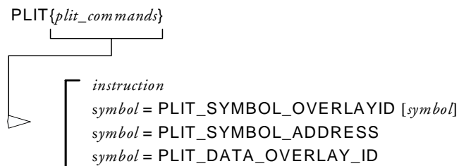
Figure 5-9. PLIT{} Command Syntax Tree
