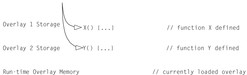
Figure 5-5. PLITs and Overlay Memory; main() Calls to Overlays
