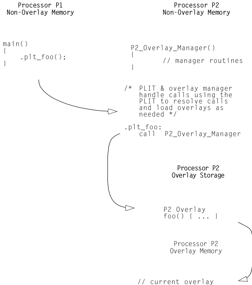
Figure 5-6. PLITs and Overlay Memory – Inter-Processor Calls
