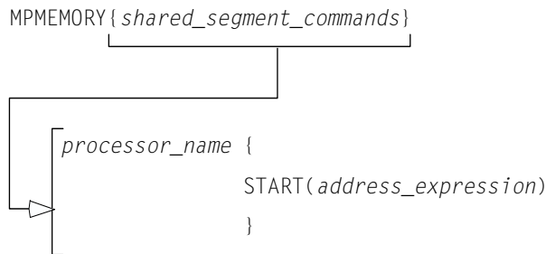
Figure 5-10. MPMEMORY{} Command Syntax Tree
