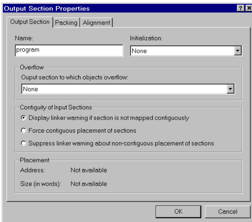
Figure 4-51. Output Section Properties Dialog Box – Output Section Tab
