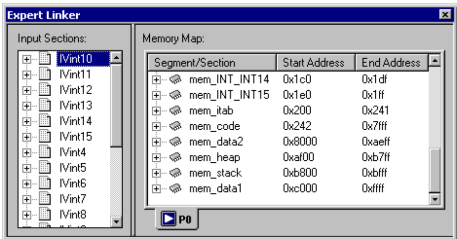
Figure 2-3. Expert Linker Window
