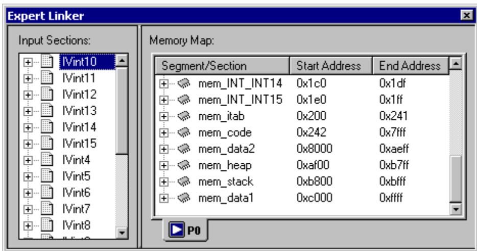
Figure 4-1. Expert Linker Window
