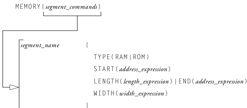
Figure 3-2. MEMORY{} Command Syntax Tree
