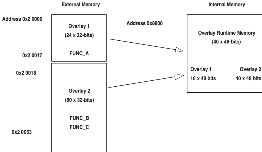
Figure 5-4. SHARC Overlay Live and Run Memory Sizes
