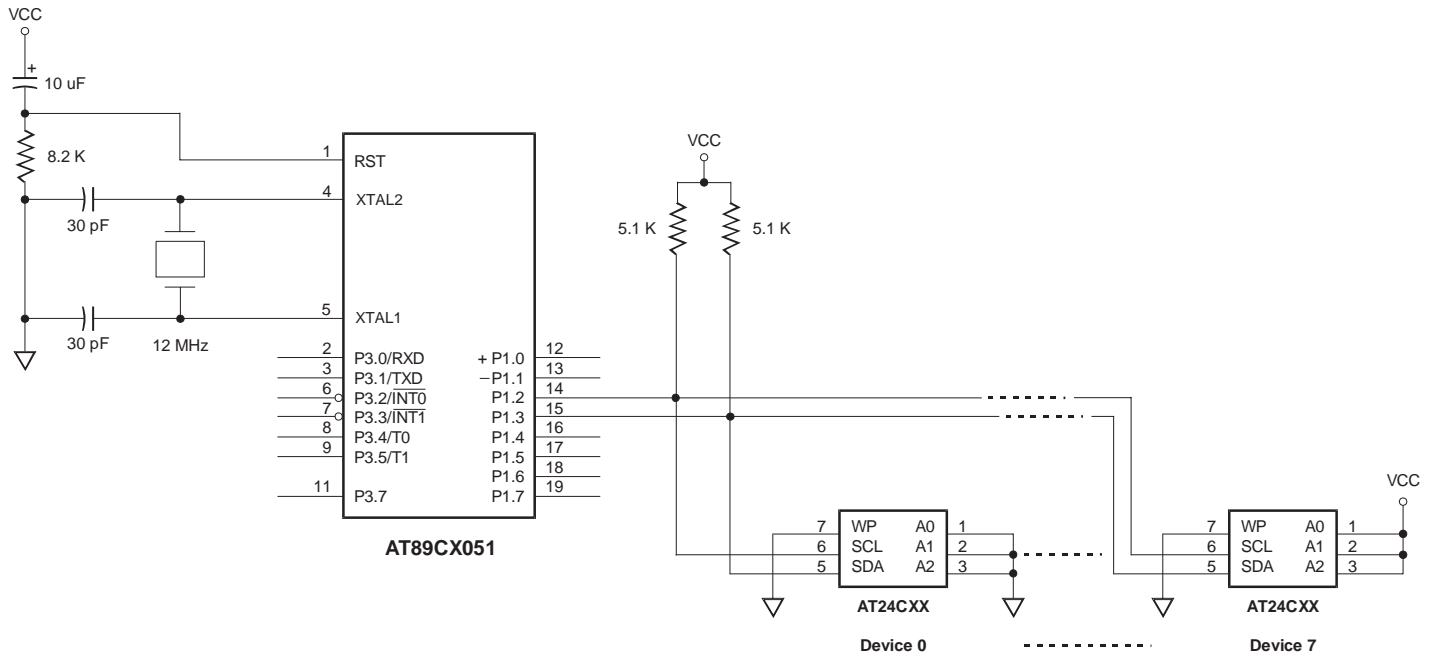
Figure 1. Typical Circuit Configuration
