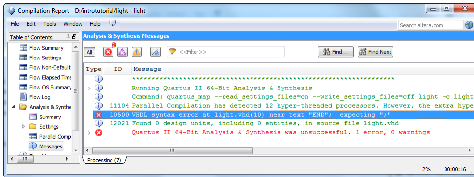
Figure 21. Error messages.
