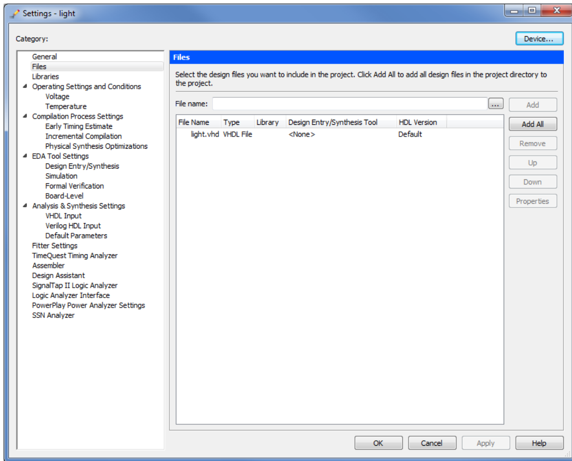
Figure 17. Settings window.
